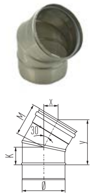
Elbow 30°
