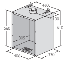
Recessed Flue Box
