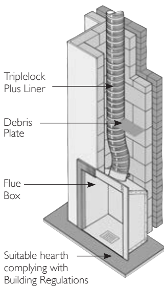
Fig. 1 Typical Triplelock Plus Installation
